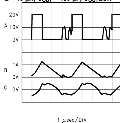
A. V_{SW} Pin Voltage, 10 V/div. B. Inductor Current, 1 A/div C. Output Ripple Voltage, 20 mV/div AC-Coupled Figure 13. Horizontal Time Base: 1 \mu s /div
