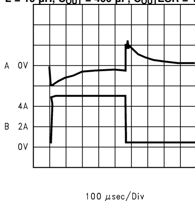
A. Output Voltage, 100 mV/div, AC-Coupled. B. Load Current: 500 mA to 5A Load Pulse Figure 14. Horizontal Time Base: 100 \mu s /div
