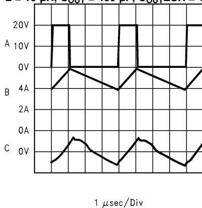
A. V_{SW} Pin Voltage, 10 V/div. B. Inductor Current, 2 A/div C. Output Ripple Voltage, 20 mV/div AC-Coupled Figure 12. Horizontal Time Base: 1 \mu s /div
