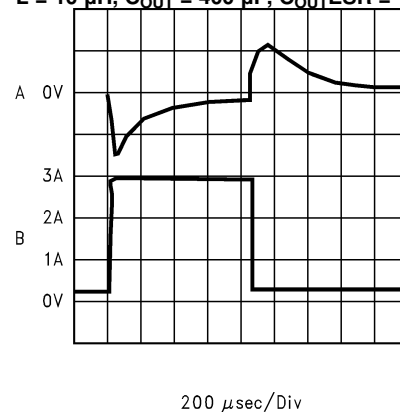
A. Output Voltage, 100 mV/div, AC-Coupled. B. Load Current: 200 mA to 3A Load Pulse Figure 15. Horizontal Time Base: 200 \mu s /div
